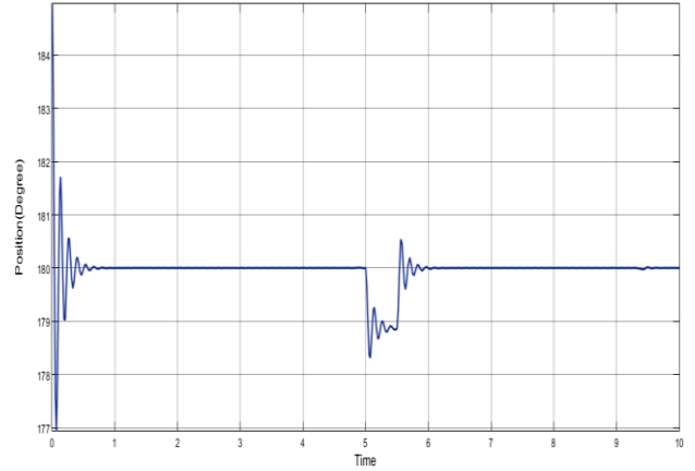
FIGURE 11. EFFECT OF DISTURBANCE ON BODY ANGEL WITH PID CONTROL
