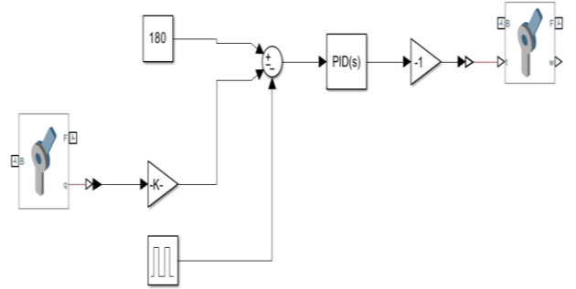
FIGURE 5. SIMSCAPE MODEL FOR PID CONTROLLER
