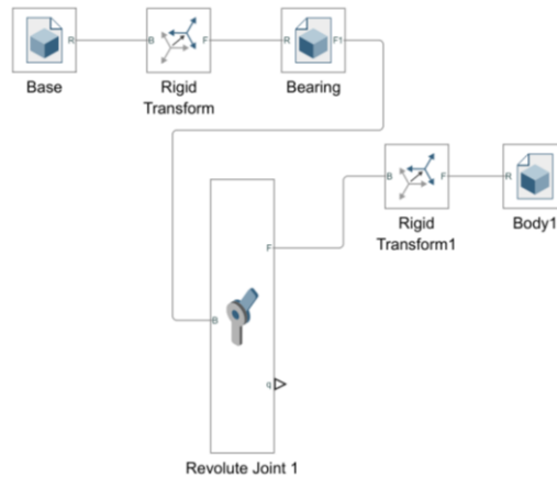
FIGURE 1. JOINT 1 CONFIGURATION, CONNECTION BETWEEN BODY AND BASE
