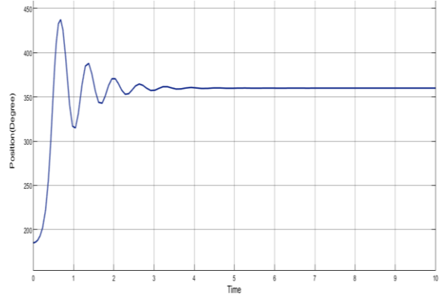
FIGURE 8. TILT ANGEL OF THE BODY OVER TIME WITHOUT PID CONTROL
