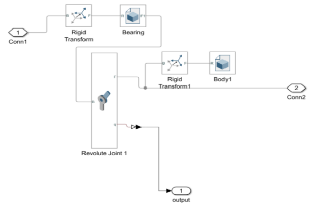
FIGURE 3. SIMSCAPE MODEL FOR BODY SUBSYSTEM
